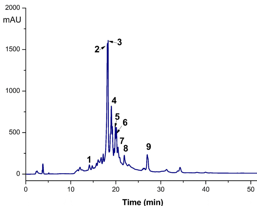
Figure 1 HPLC-DAD (220 nm) finger printing of the LPG from Ligustrum purpurascens . Compounds 1–9
