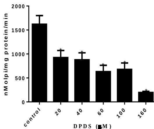
Figure 4 Effects of DPDS on basal \text{Na}^+/\text{K}^+ -ATPase activity in rat brain homogenate. Data depict mean \pm SEM of three independent
